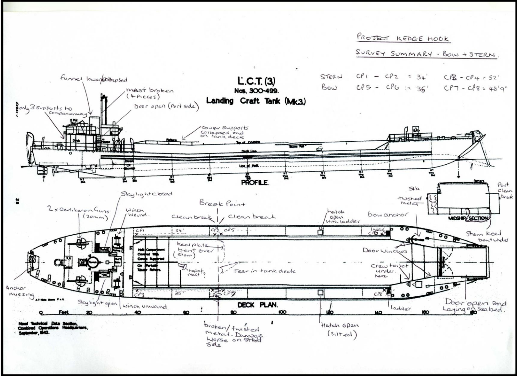
Figure 22 Annotated ship's plan with key features observed.
